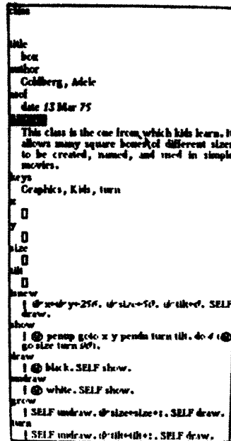
FIGURE 11.34 Retrieved HyperDocument
