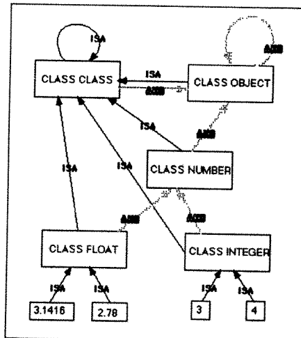
FIGURE 11.54 Smalltalk-76 Metaphysics
