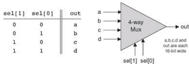
Figure 1.10 4-way multiplexor. The width of the input and output buses may vary.
