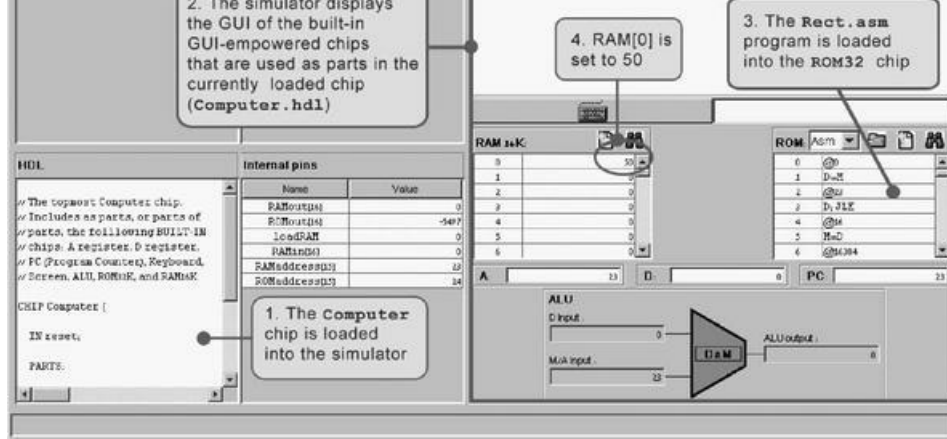
Figure 5.11 Testing the Computer chip on the hardware simulator. The Rect program draws a rectangle of width 16 pixels and length RAM[0] at the top left of the screen. Note that the program is correct. Thus, if it does not work properly, it means that the computer platform on which it runs (Computer.hdl and/or some of its lower-level parts) is buggy.
