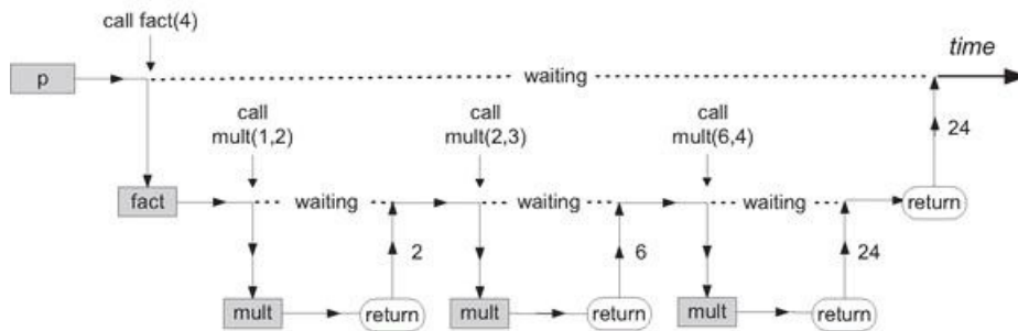
Figure 8.7 The life cycle of function calls. An arbitrary function p calls function fact, which then calls mult several times. Vertical arrows depict transfer of control from one function to another. At any given point in time, only one function is running, while all the functions up the calling chain are waiting for it to return. When a function returns, the function that called it resumes its execution.
