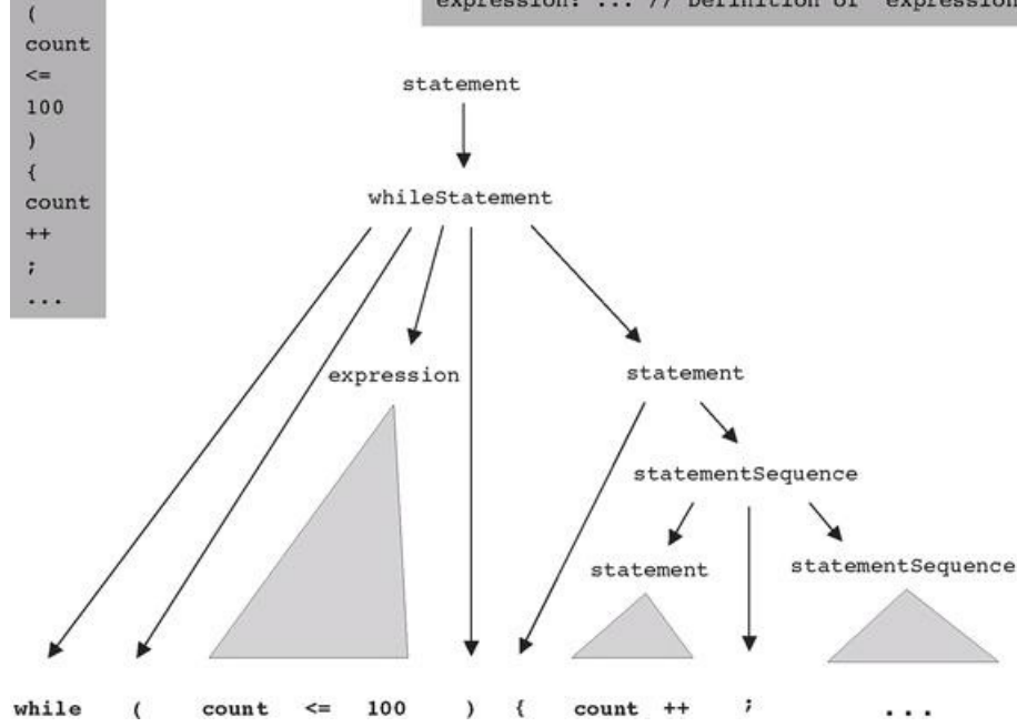
Figure 10.4 Parse tree of a program segment according to a grammar segment. Solid triangles represent lower-level parse trees.
