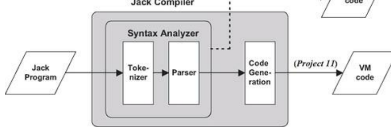
Figure 10.1 The Jack Compiler. The project in chapter 10 is an intermediate step, designed to localize the development and unit-testing of the syntax analyzer module.
