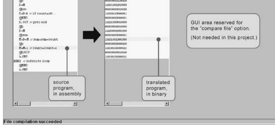
Figure 4.7 The visual assembler supplied with the book.
