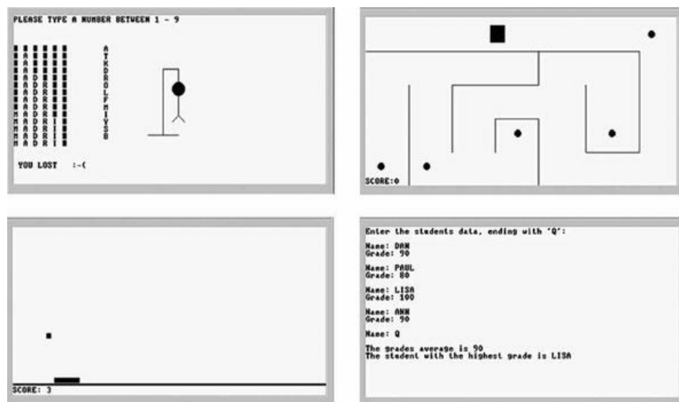
Figure 9.11 Screen shots of sample Jack applications, running on the Hack computer. Hangman, Maze, Pong, and a simple data processing program.
