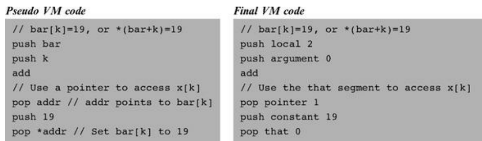
Figure 11.2 Array processing. The Hack VM code (right) follows the conventions described in section 7.2.6.
