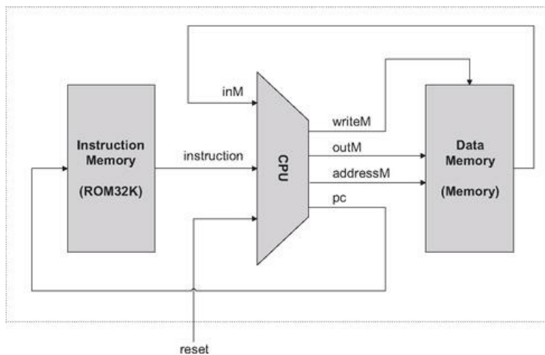
Figure 5.10 Proposed implementation of the topmost Computer chip.
