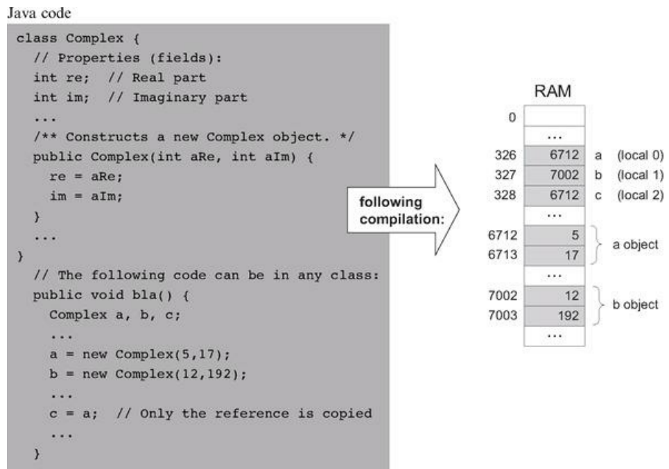
Figure 11.3 Objects handling. Since memory allocations are run-time dependent, all the shown addresses are arbitrary examples.
