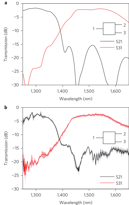
Figure 4 | S-parameters for the device, where S_{ij} is the transmission from port j to port i . a , b , Plots of transmission from input port 1 to output ports 2 and 3: S-parameters simulated using FDTD simulations ( a ); measured S-parameters simulated using three identical devices ( b ). Shaded areas indicate minimum and maximum measured values across all measured devices, and solid lines indicate the average values. The measured devices exhibit relatively low peak insertion losses of -1.8 dB and -2.4 dB in the 1,300 nm and 1,550 nm bands, and broad 3 dB bandwidths of 100 nm and 170 nm, respectively. Crosstalk is less than -11 dB throughout both bands. The insertion losses and crosstalk of the device are somewhat degraded with respect to the simulated values due to fabrication imperfections.
